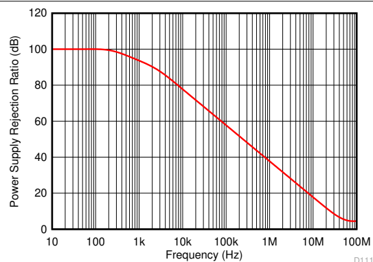
Figure 6-51. Power Supply Rejection Ratio vs Frequency
