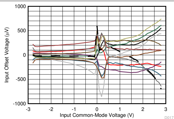
Figure 6-41. Input Offset Voltage vs Input Common-Mode Voltage
